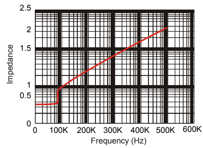
Figure 7. Dynamic Impedance
