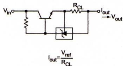
Figure 5. Constant Current Source
