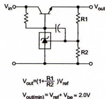
Figure 4. Series Pass Regulator
