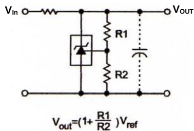
Figure 1. Shunt Regulator
