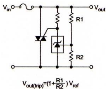
Figure 7. TRIAC Crowbar
