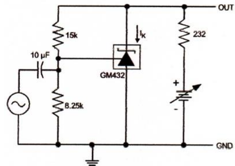
Figure 14. Test Circuit – Small Signal Gain and Phase
